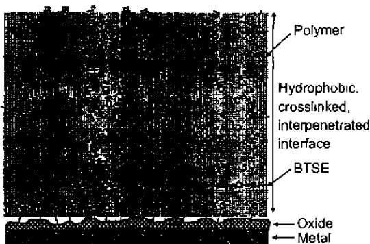
Fig. 1 Model for bonding mechanism of BTSE films to polymers
