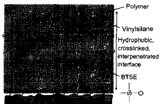
Fig. 2 Interface between polymer and metal modified by a 2-step BTSE-VS silane treatment
